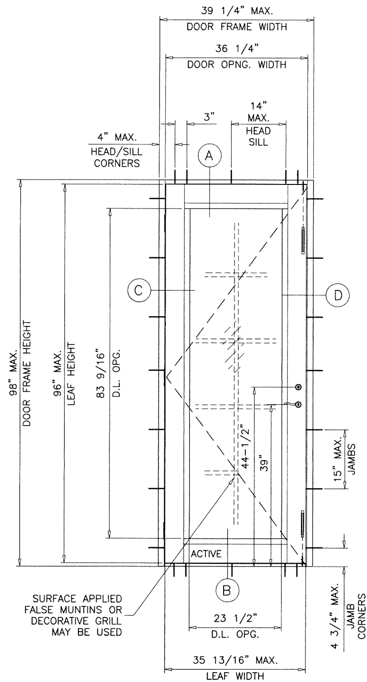
TYPICAL ELEVATION ( X )
