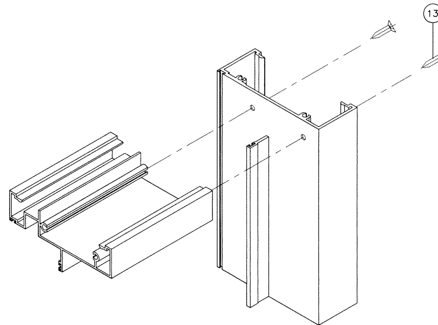
DOOR/SIDELITE TOP CORNER
